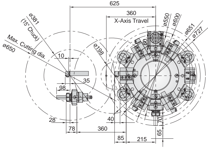
FBL-460MC Tool Interference BMT 75
