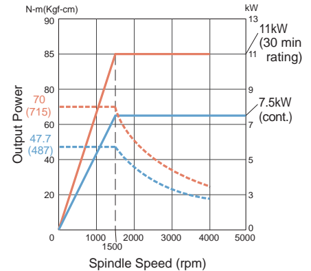
FBL-360MC/460MC Power Tool Torque
